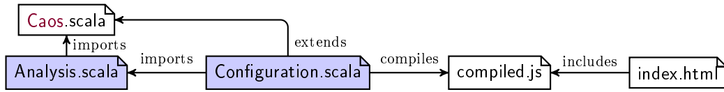
Figure 2: Architecture of a Scala project that uses Caos
