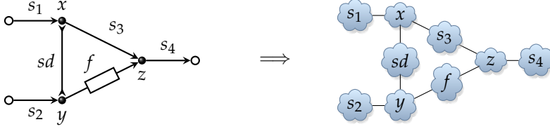
Figure 6.10: Encoding of a Reo connector as a Dreams configuration.
