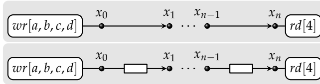
Figure 7.8: Sequences of n Sync channels (above) and FIFO 1 channels (below).
