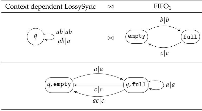
Figure 3.8: Product of the normalised \mathcal{R}\text{eo} automata of the context dependent LossySync and FIFO 1 channels.
