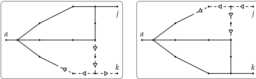
Figure 4.3: Flow colourings for the priority exclusive-router connector.
