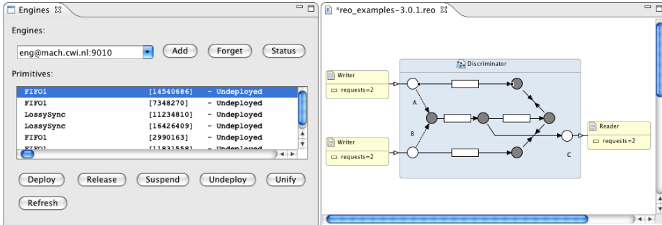
Figure 7.16: Deployment plug-in for the Dreams framework for Reo (left) and ECT’s editor (right).
