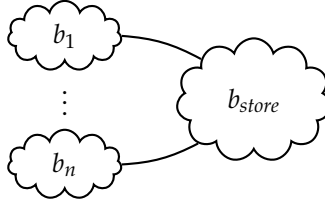
Figure 3.10: Outline of the behavioural automata for the tuple space term P_1 \oplus \dots \oplus P_n \oplus T .
