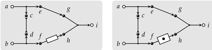
Figure 4.4: Two possible states of the alternating coordinator.
