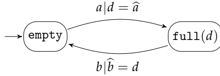
Figure 5.2: Constraint Automata for the \text{FIFO}_1 channel
