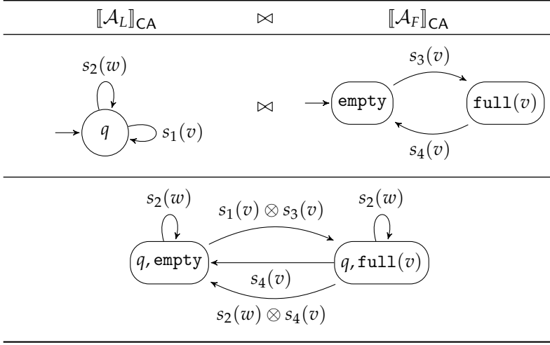
Figure 3.7: Composition of \llbracket \mathcal{A}_L \rrbracket_{\text{CA}} and \llbracket \mathcal{A}_F \rrbracket_{\text{CA}} , for any v, w \in \mathbb{D} .
