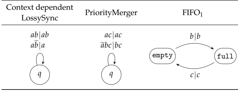
Figure 2.5: Normalised \mathcal{R}\text{eo} automata of the context dependent LossySync, the priority merger, and the FIFO 1 primitives.
