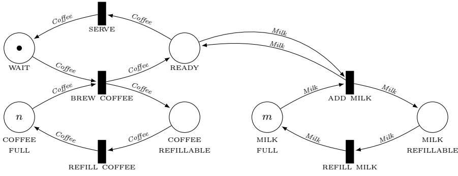
Fig. 3: Arc-labelled FN of the product line \{\{Coffee\}, \{Coffee, Milk\}\} . Each arc has an application condition attached.
