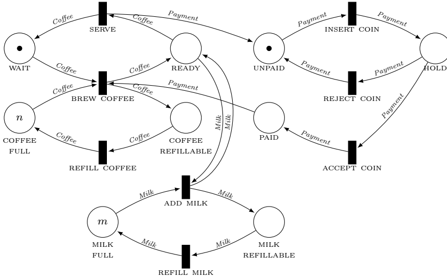
Fig. 10: FN model of an SPL over the feature set \{Coffee, Payment, Milk\} obtained by sequential application of the delta nets for the features Payment (Fig. 8c) and Milk (Fig. 8b).
