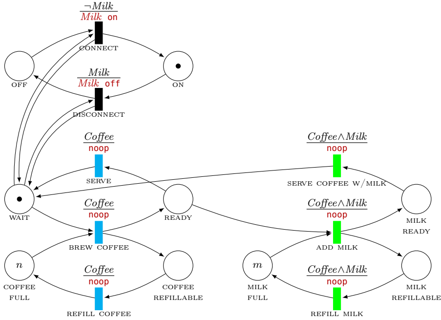
Fig. 6: DFN (initial state) of a dynamically reconfigurable product line. Whenever transition DISCONNECT fires, feature Milk is switched off, disabling all transitions that are conditioned on Milk . It is enabled again by firing CONNECT.
